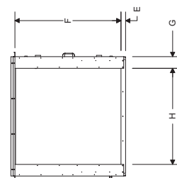
INTAKE VIEW
