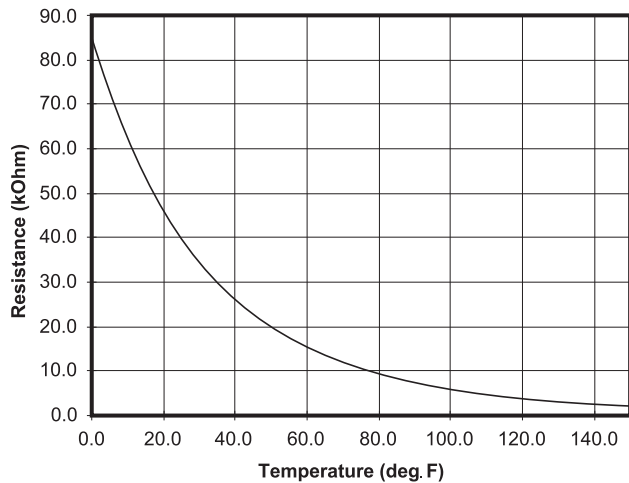
Chart 1: Thermistor Nominal Resistance
