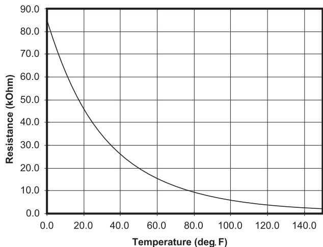
Chart 2: Thermistor Nominal Resistance
