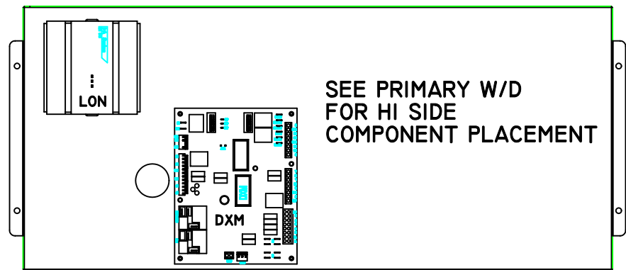
CONTROL BOX LAYOUT LOW SIDE
