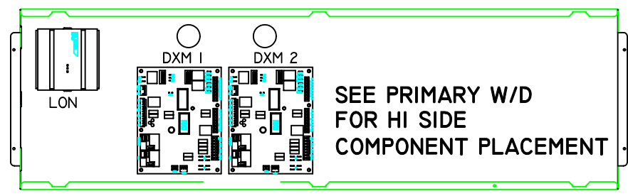
CONTROL BOX LAYOUT LOW SIDE
