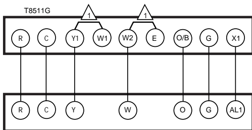
CXM TERMINALS
