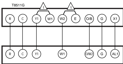
DXM TERMINALS
