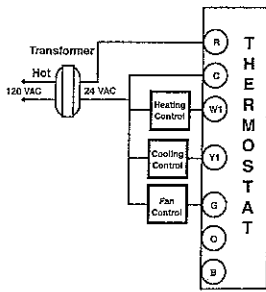
HEAT/COOL 4-WIRE SINGLE TRANSFORMER
