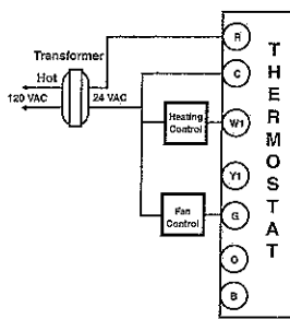
HEAT ONLY 3-WIRE SINGLE TRANSFORMER
