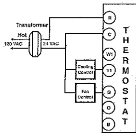
COOL ONLY 3-WIRE SINGLE TRANSFORMER
