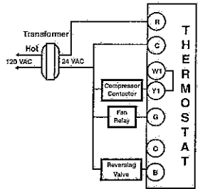
HEAT PUMP WITH HEAT ACTIVE REVERSING VALVE
