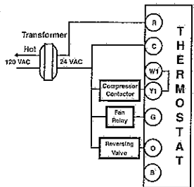
HEAT PUMP WITH COOL ACTIVE REVERSING VALVE
