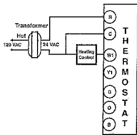
HEAT ONLY 2-WIRE SINGLE TRANSFORMER
