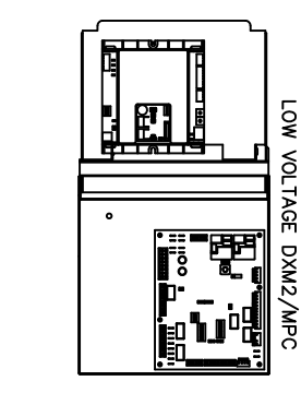
CONTROL BOX LAYOUT LOW VOLTAGE DXM2/MPC
