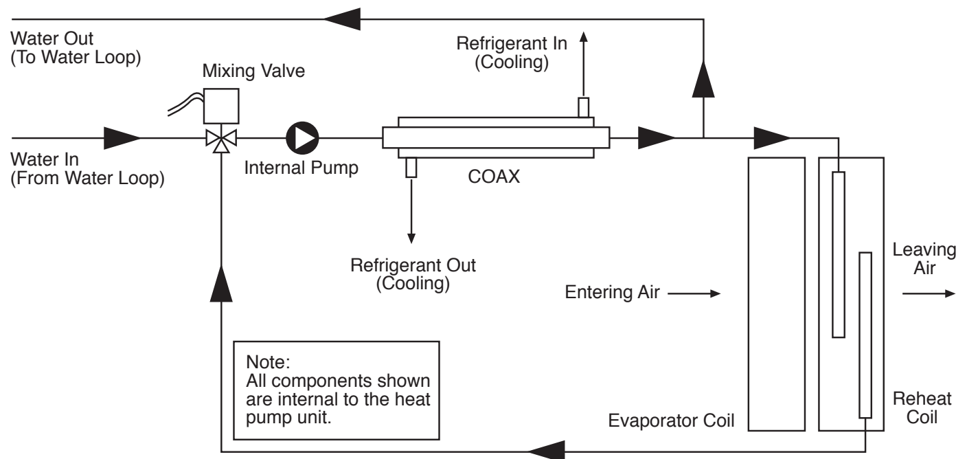
Figure 1: ClimaDry Schematic
